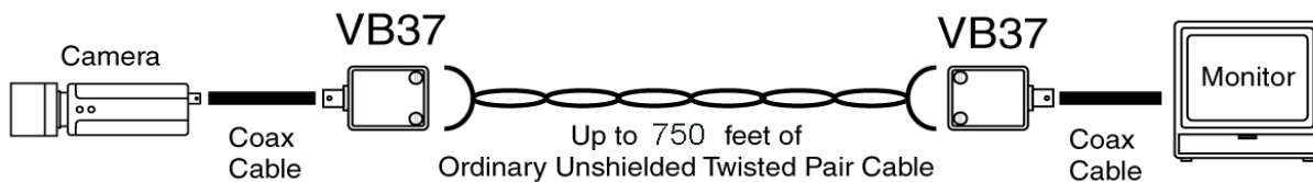
Basic Twisted Pair Video Transmission System
